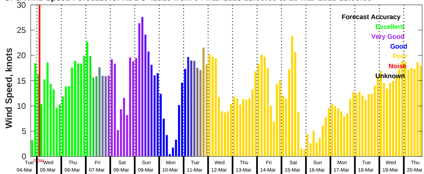
GFS Wind Speed Forecast for NDBC 42020 from 04-Mar-2025 18:00:00 to 20-Mar-2025 18:00:00
