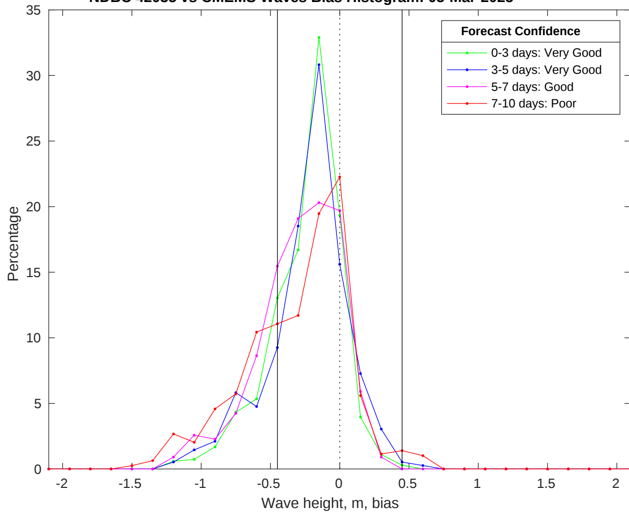
NDBC 42035 vs CMEMS Waves Bias Histogram: 05-Mar-2025
