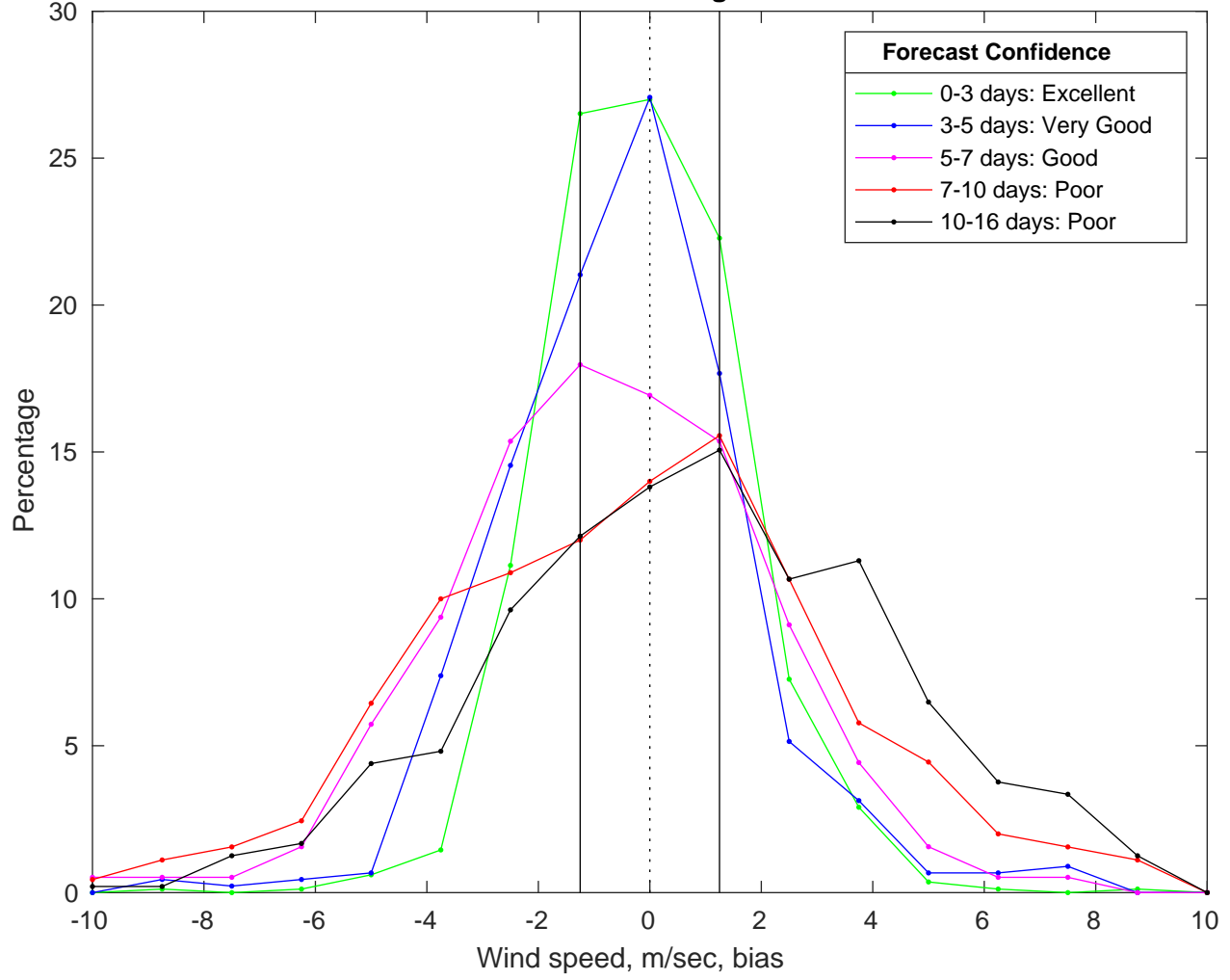
NDBC 42035 vs GFS Winds Bias Histogram: 05-Mar-2025
