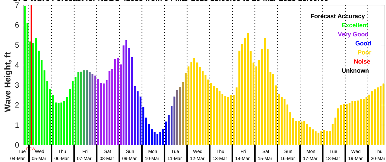
GFS Wave Forecast for NDBC 42035 from 04-Mar-2025 18:00:00 to 20-Mar-2025 18:00:00
