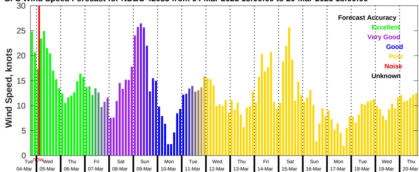
GFS Wind Speed Forecast for NDBC 42035 from 04-Mar-2025 18:00:00 to 20-Mar-2025 18:00:00
