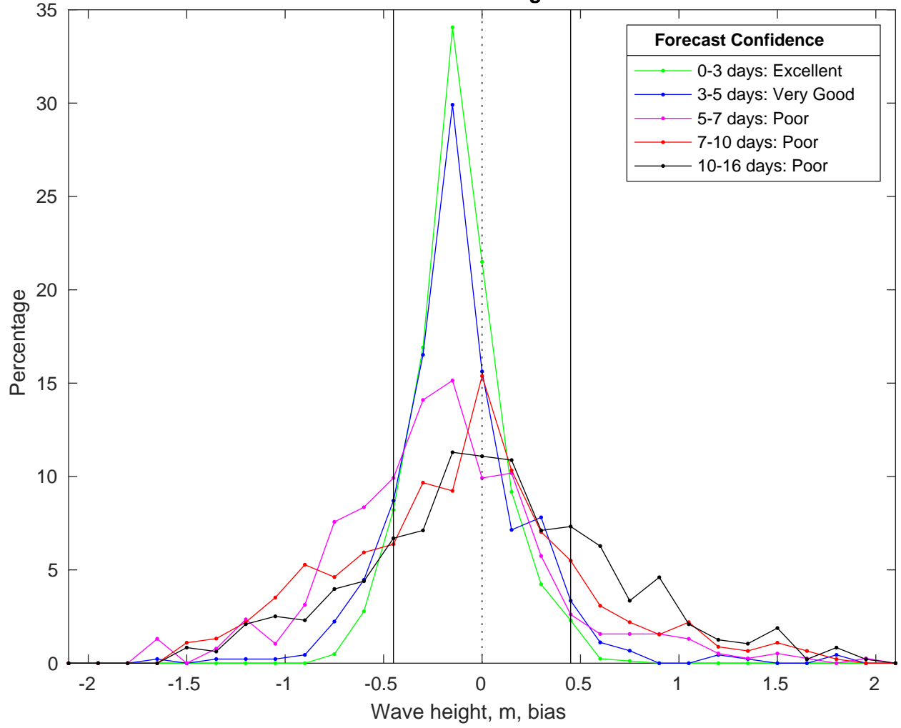
NDBC 42036 vs GFS Waves Bias Histogram: 05-Mar-2025
