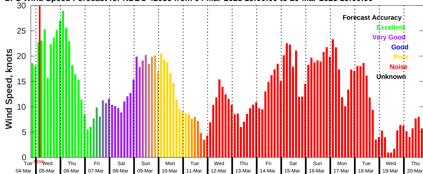
GFS Wind Speed Forecast for NDBC 42036 from 04-Mar-2025 19:00:00 to 20-Mar-2025 19:00:00
