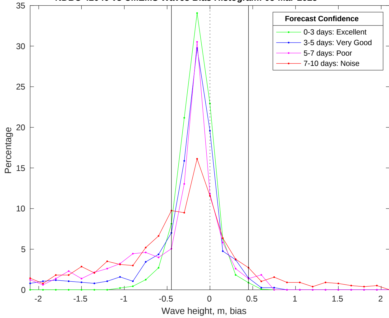
NDBC 42040 vs CMEMS Waves Bias Histogram: 05-Mar-2025
