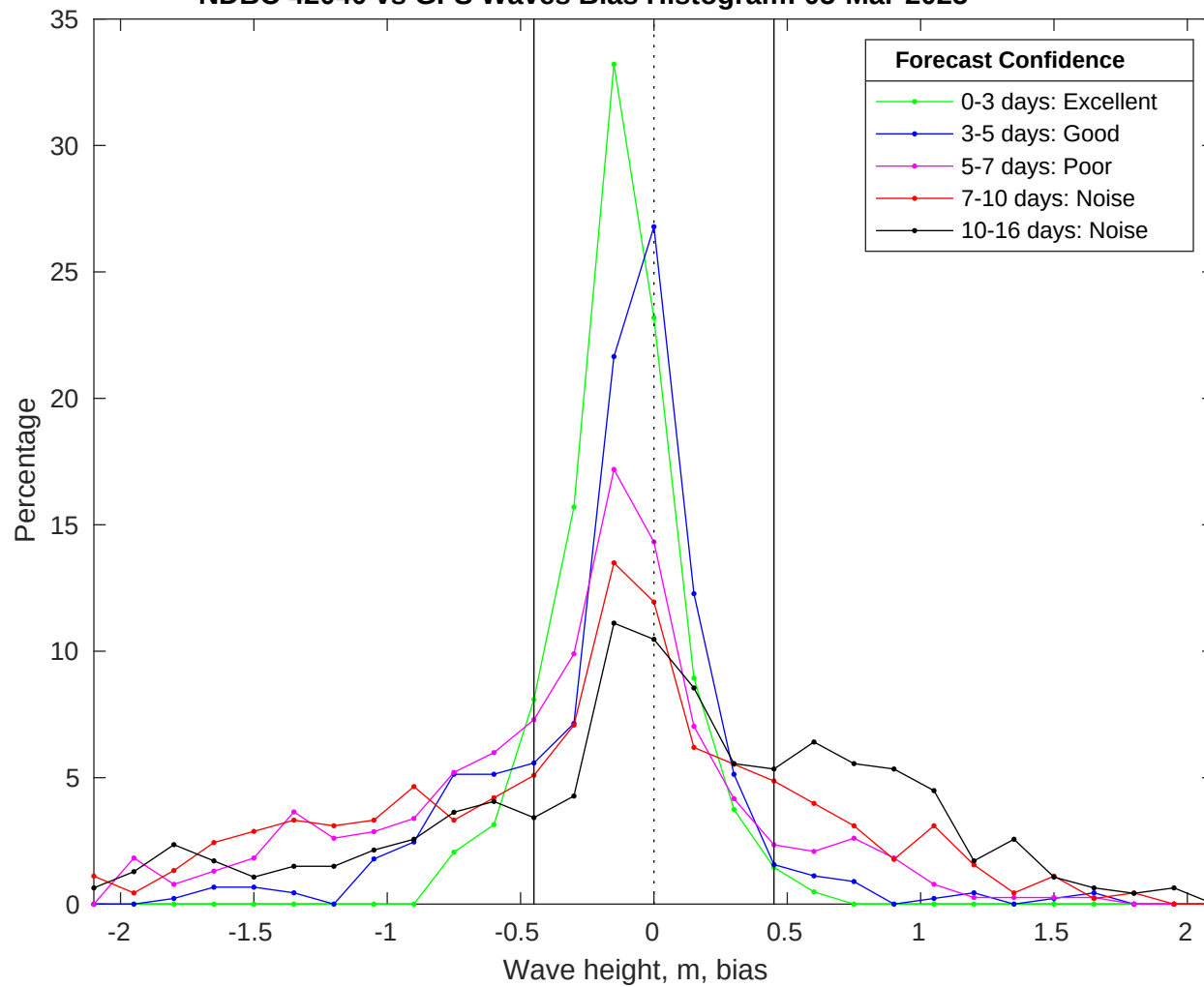
NDBC 42040 vs GFS Waves Bias Histogram: 05-Mar-2025
