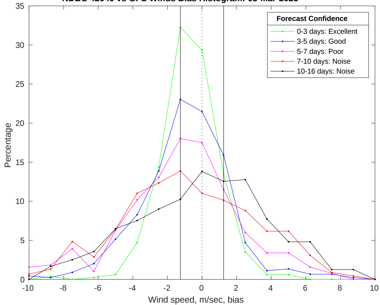
NDBC 42040 vs GFS Winds Bias Histogram: 05-Mar-2025
