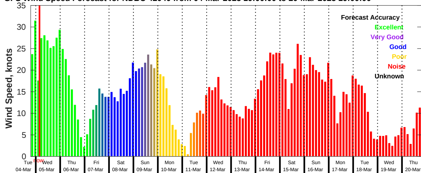
GFS Wind Speed Forecast for NDBC 42040 from 04-Mar-2025 19:00:00 to 20-Mar-2025 19:00:00
