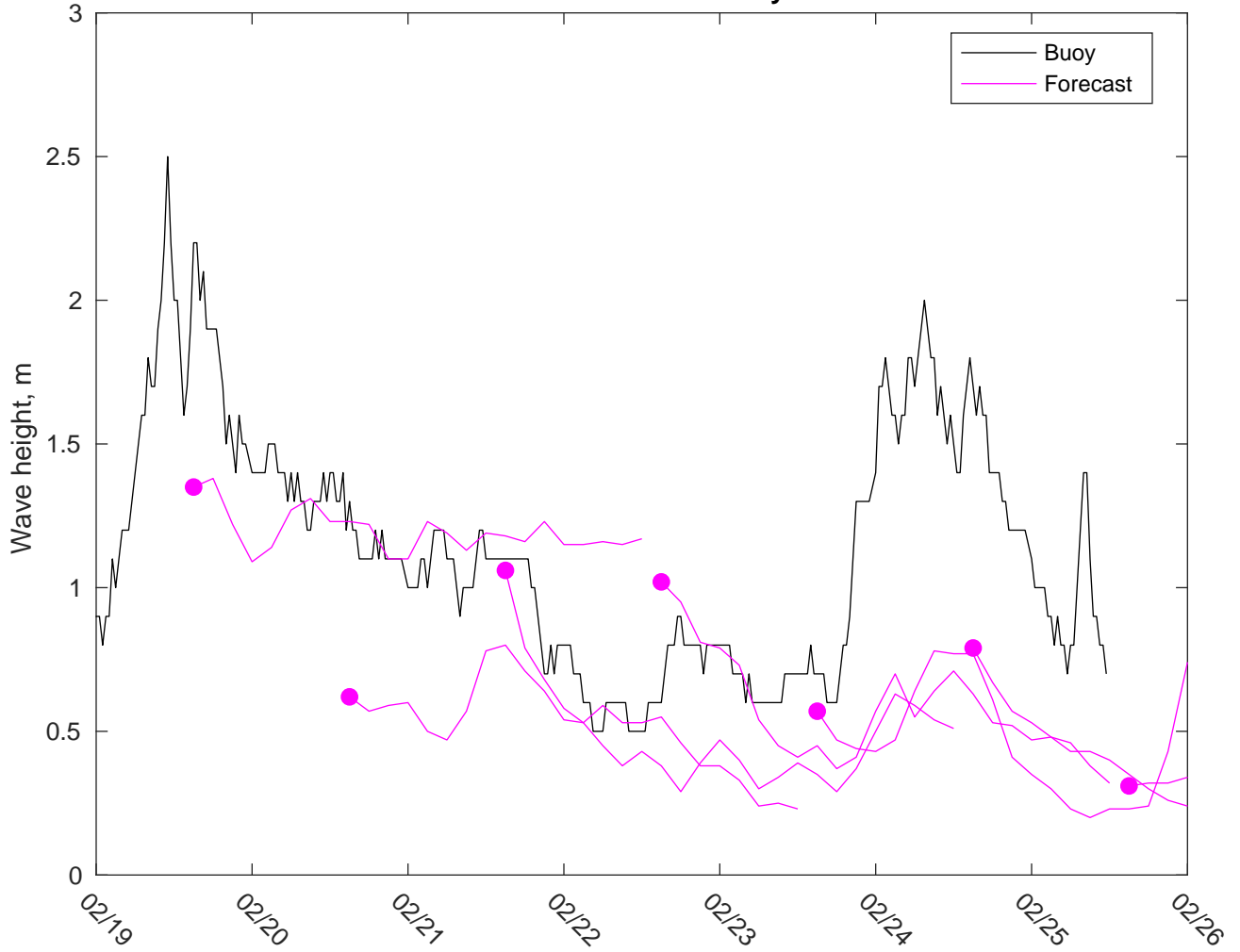
NDBC 42084 vs GFS Waves: 7 to 10 day forecast
