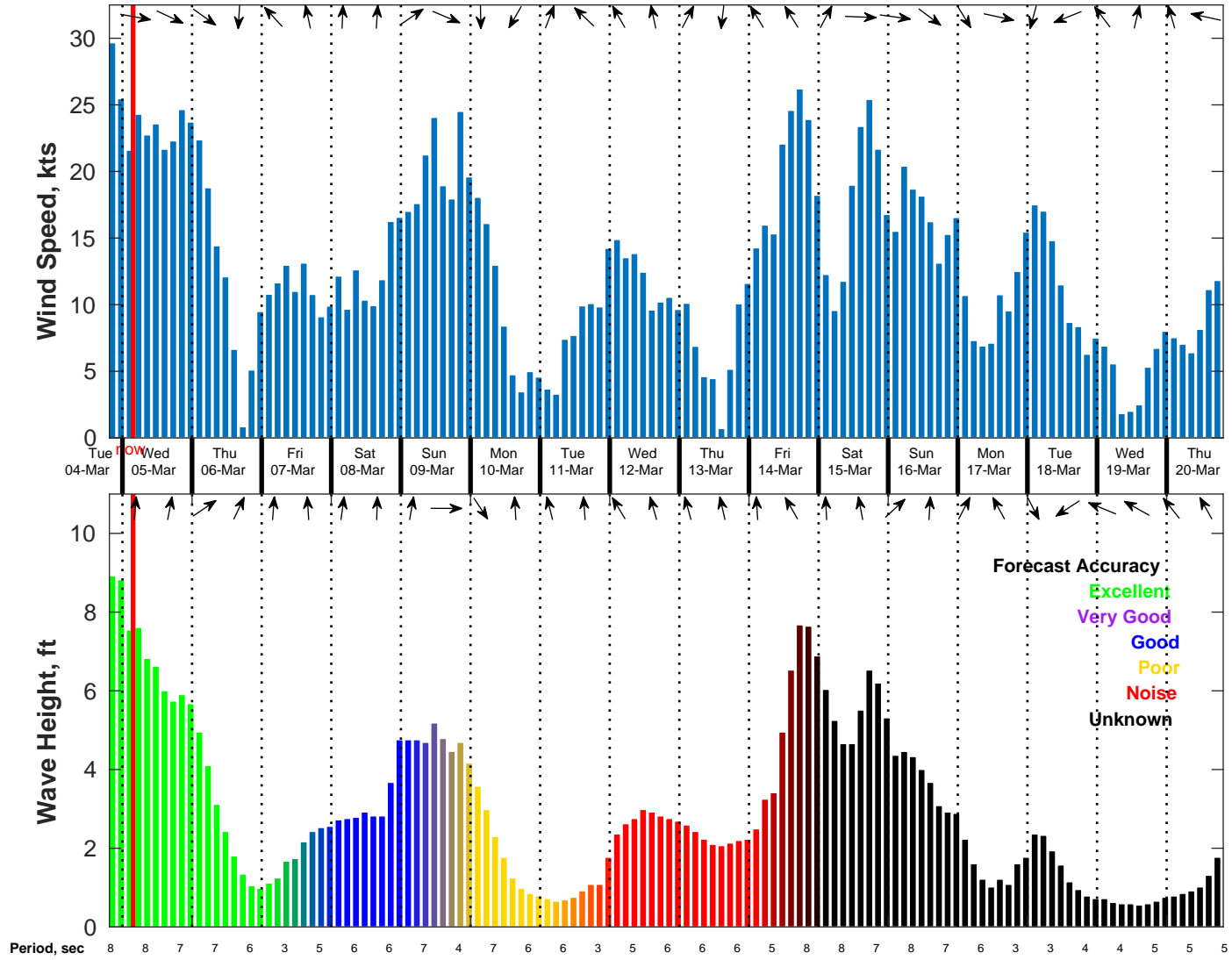
Wind & Wave Forecast for NDBC 42084 from 04-Mar-2025 19:00:00 to 20-Mar-2025 19:00:00
