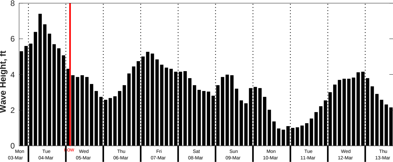
CMEMS Wave Forecast for NDBC 42092 from 03-Mar-2025 18:00:00 to 13-Mar-2025 18:00:00
