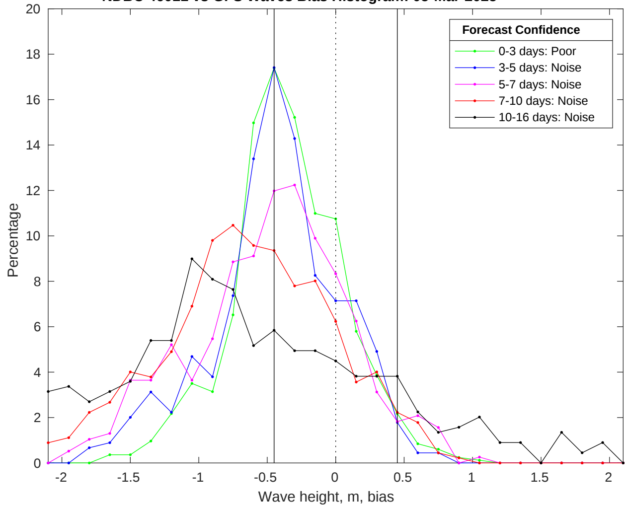
NDBC 46011 vs GFS Waves Bias Histogram: 05-Mar-2025
