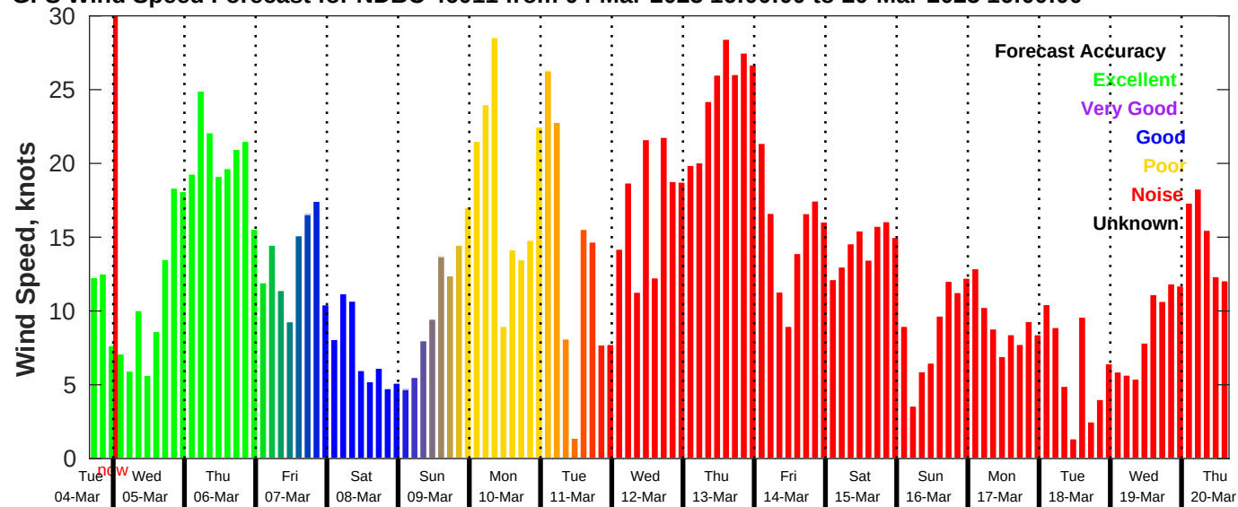
GFS Wind Speed Forecast for NDBC 46011 from 04-Mar-2025 16:00:00 to 20-Mar-2025 16:00:00
