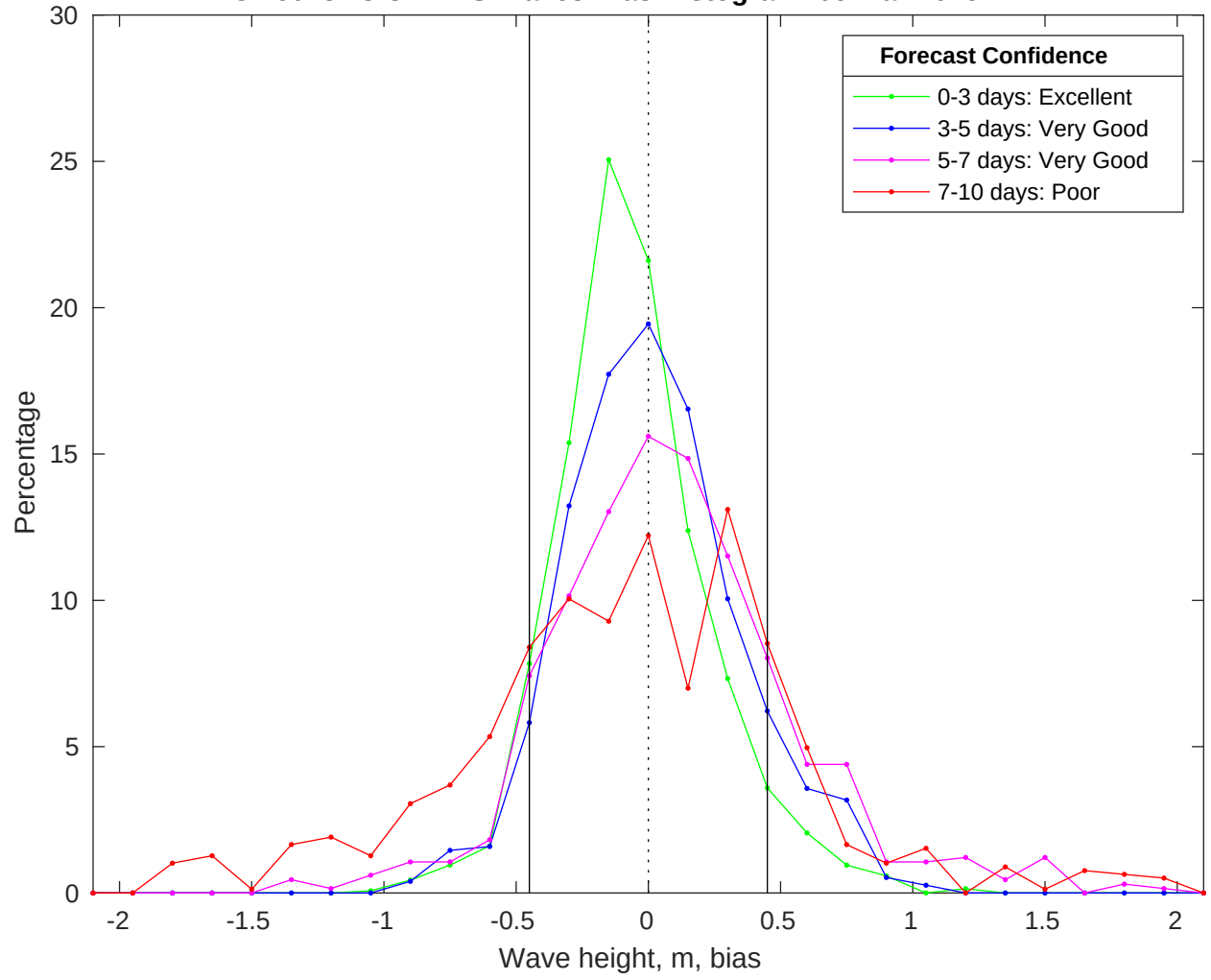
NDBC 46028 vs CMEMS Waves Bias Histogram: 05-Mar-2025
