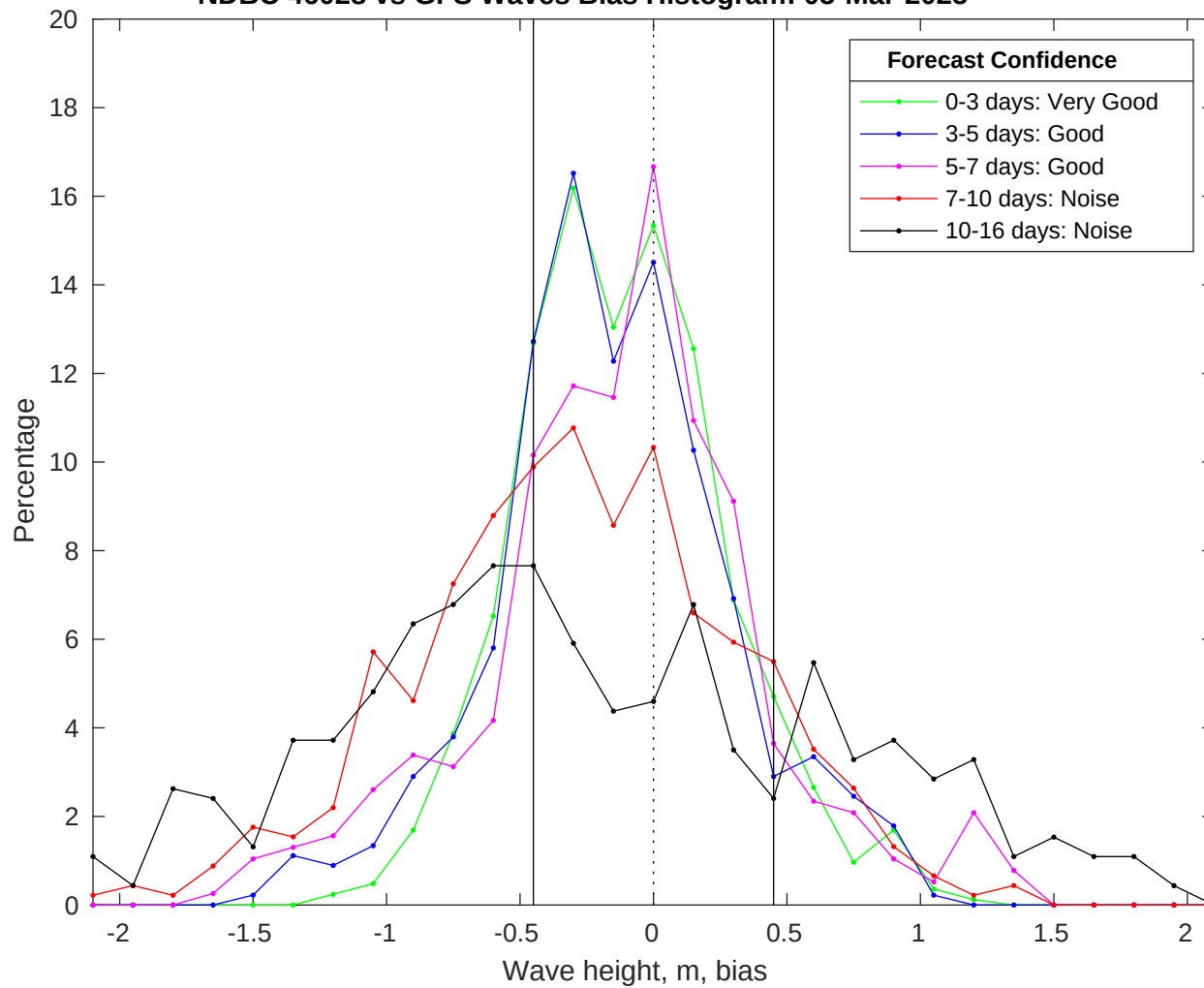
NDBC 46028 vs GFS Waves Bias Histogram: 05-Mar-2025
