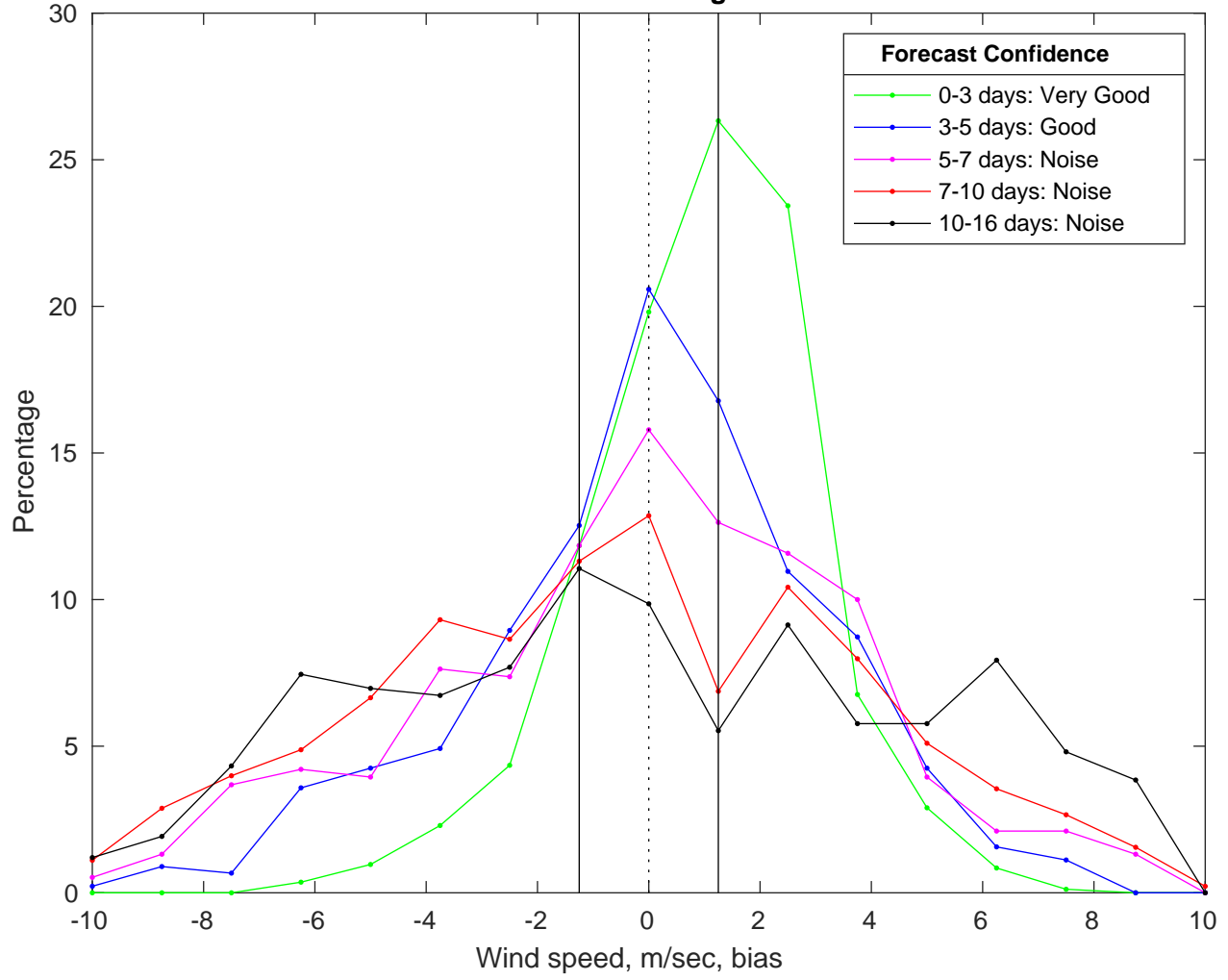
NDBC 46028 vs GFS Winds Bias Histogram: 05-Mar-2025
