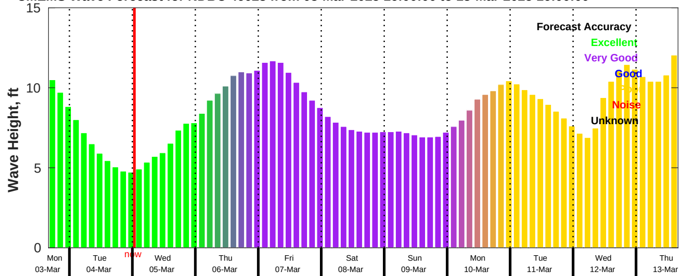
CMEMS Wave Forecast for NDBC 46028 from 03-Mar-2025 16:00:00 to 13-Mar-2025 16:00:00
