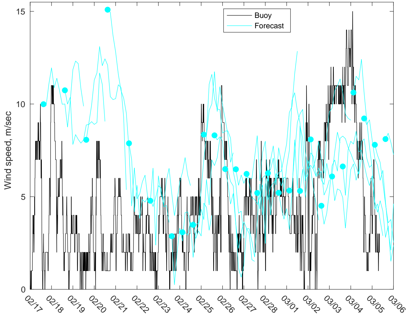
NDBC 46053 vs GFS Winds: 5 to 7 day forecast
