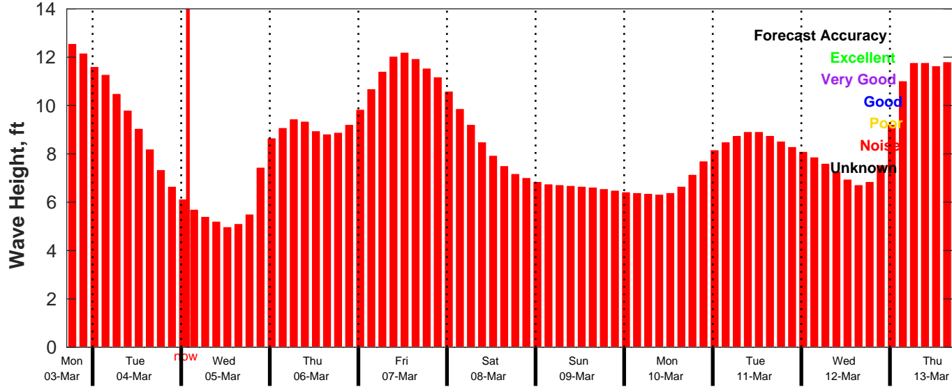
CMEMS Wave Forecast for NDBC 46053 from 03-Mar-2025 17:00:00 to 13-Mar-2025 17:00:00
