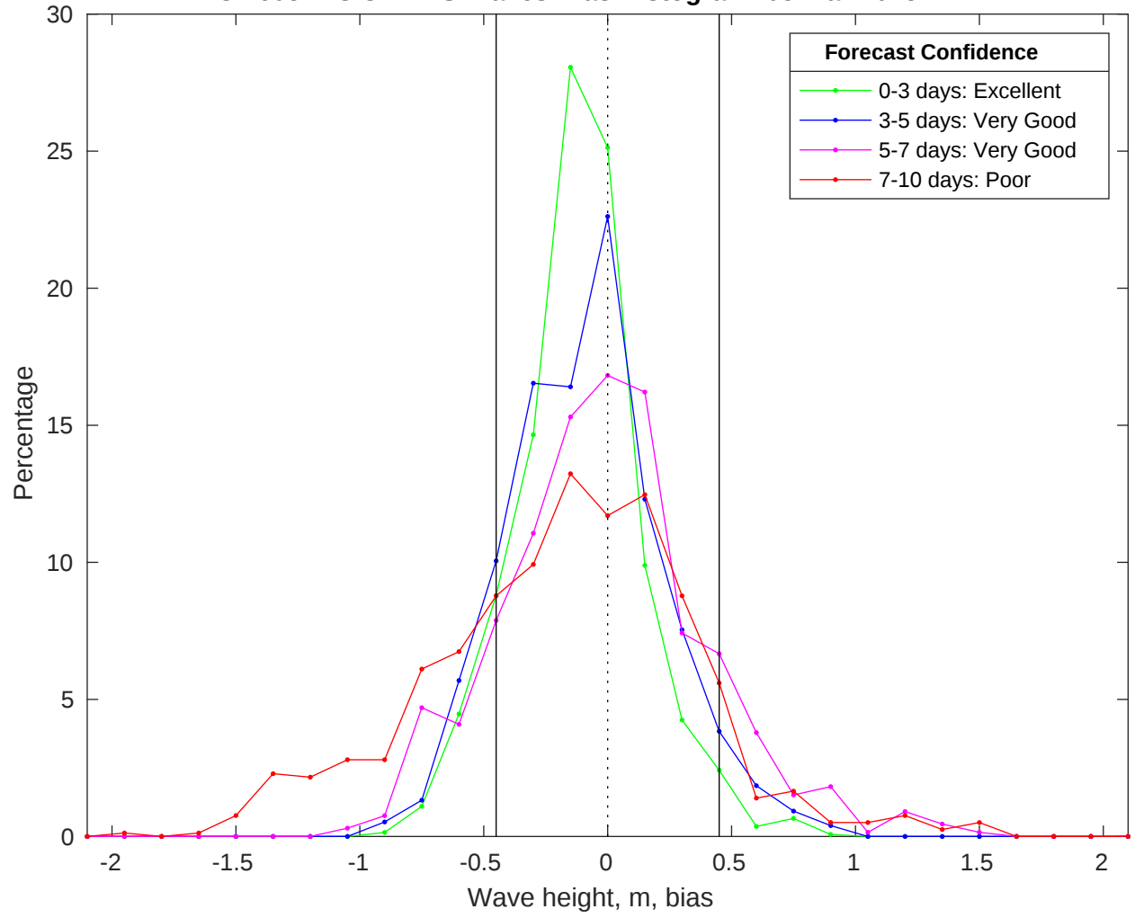
NDBC 46054 vs CMEMS Waves Bias Histogram: 05-Mar-2025
