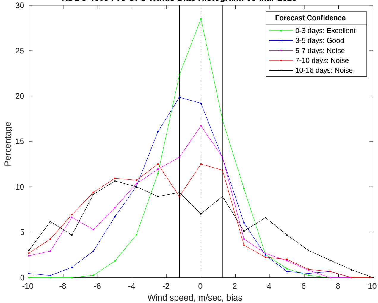
NDBC 46054 vs GFS Winds Bias Histogram: 05-Mar-2025
