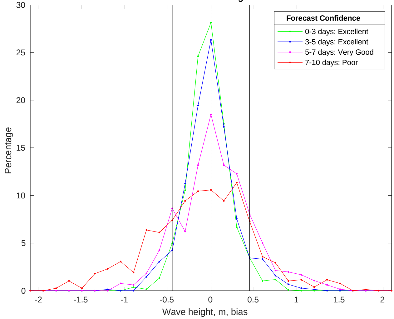
NDBC 46069 vs CMEMS Waves Bias Histogram: 05-Mar-2025
