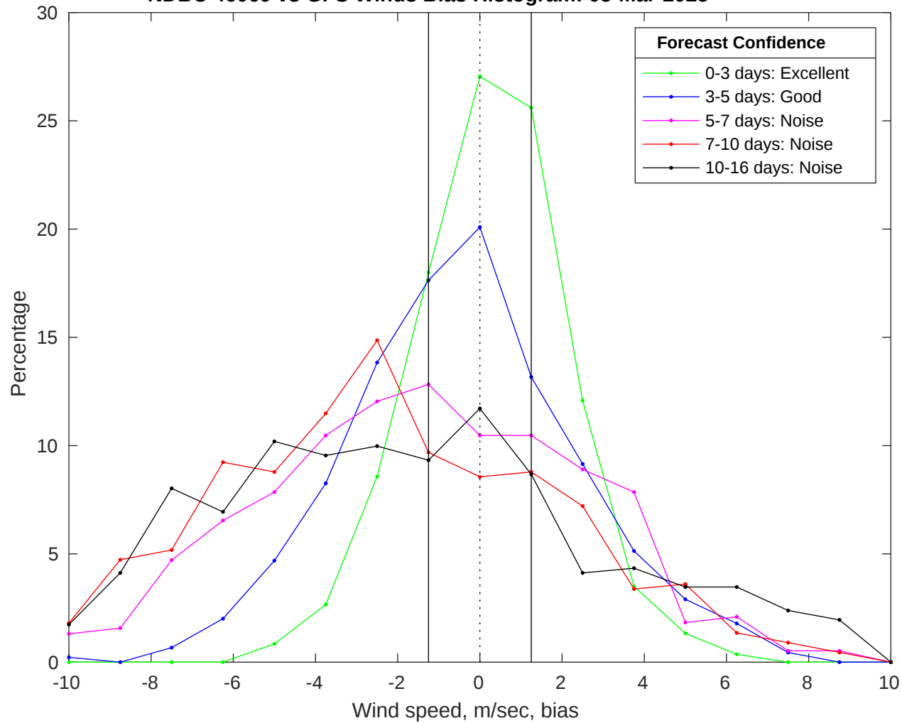
NDBC 46069 vs GFS Winds Bias Histogram: 05-Mar-2025
