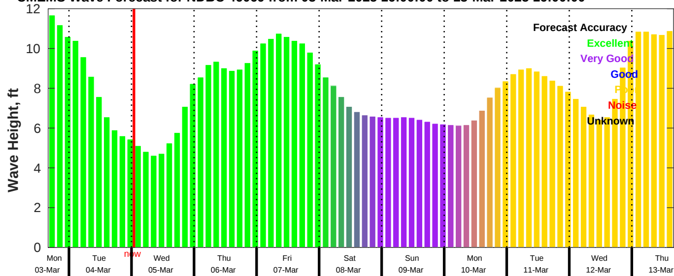
CMEMS Wave Forecast for NDBC 46069 from 03-Mar-2025 16:00:00 to 13-Mar-2025 16:00:00
