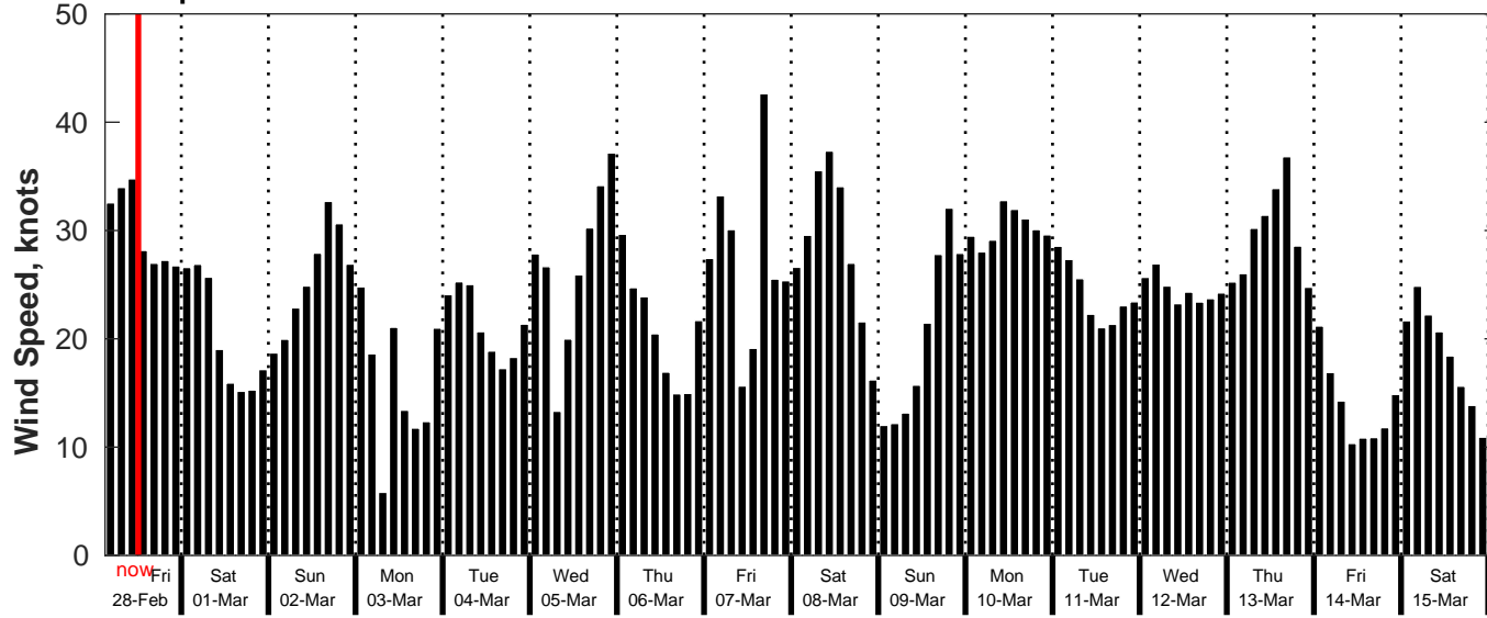
GFS Wind Speed Forecast for NDBC 46246 from 28-Feb-2025 03:00:00 to 16-Mar-2025 03:00:00
