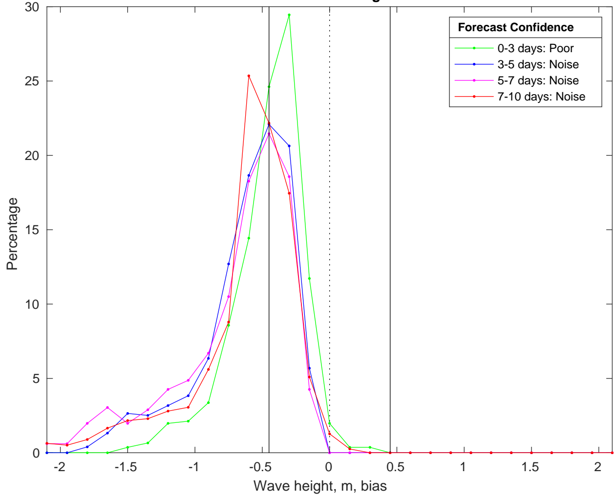
NDBC 51209 vs CMEMS Waves Bias Histogram: 05-Mar-2025
