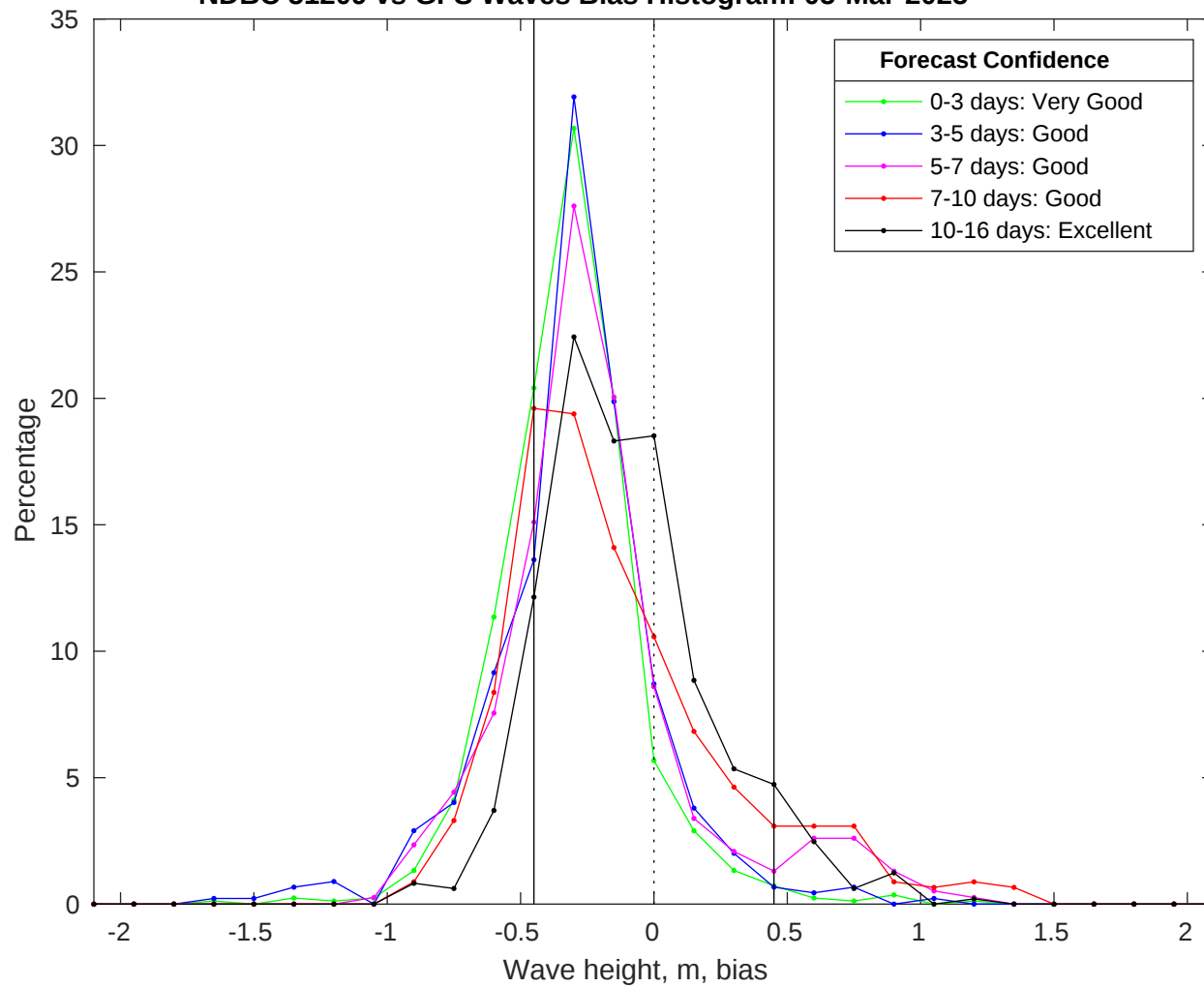
NDBC 51209 vs GFS Waves Bias Histogram: 05-Mar-2025
