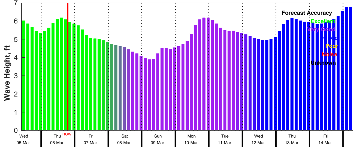
CMEMS Wave Forecast for NDBC 52211 from 04-Mar-2025 10:00:00 to 14-Mar-2025 10:00:00
