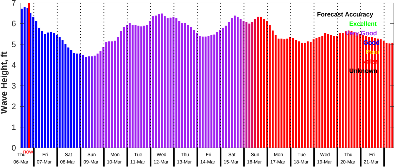
GFS Wave Forecast for NDBC 52211 from 05-Mar-2025 10:00:00 to 21-Mar-2025 10:00:00
