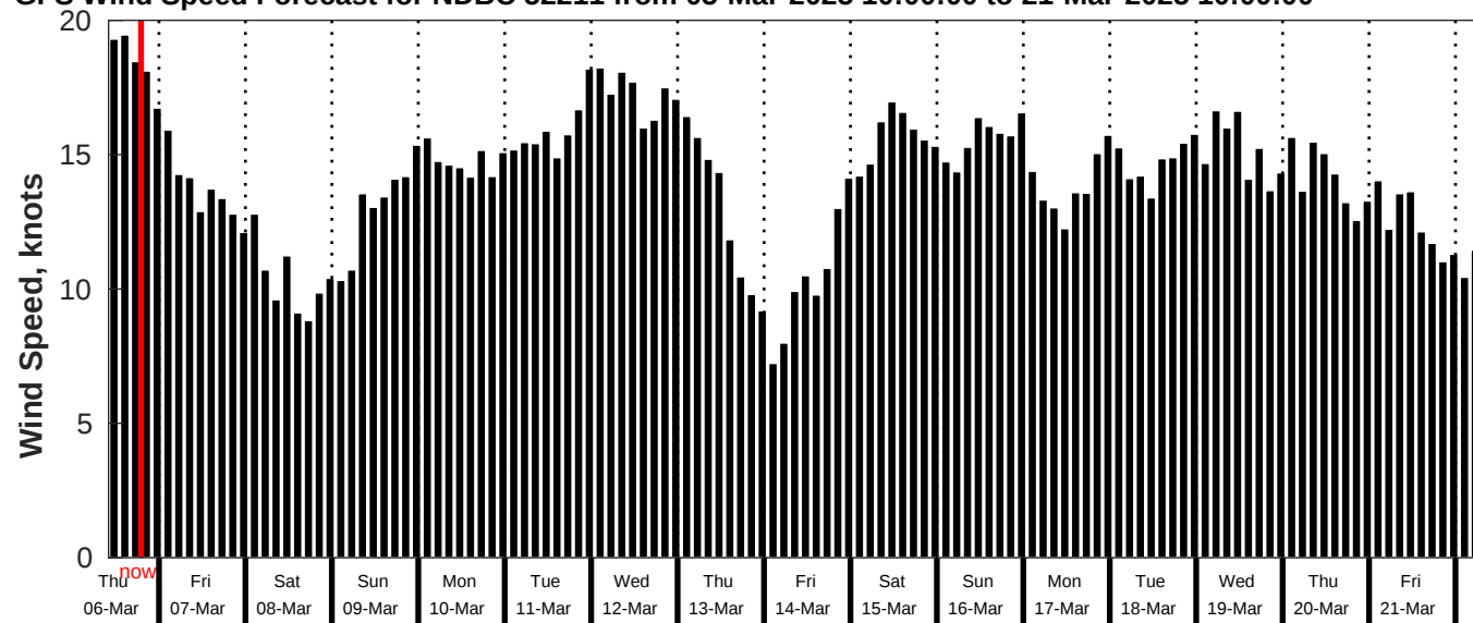
GFS Wind Speed Forecast for NDBC 52211 from 05-Mar-2025 10:00:00 to 21-Mar-2025 10:00:00
