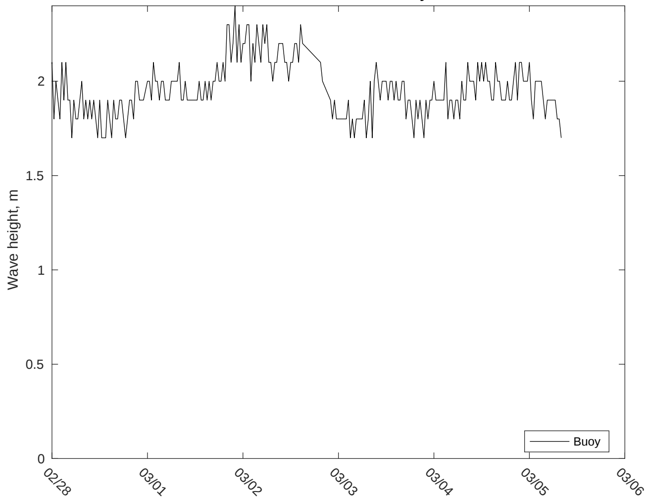
NDBC 52212 vs CMEMS Waves: 10 to 16 day forecast
