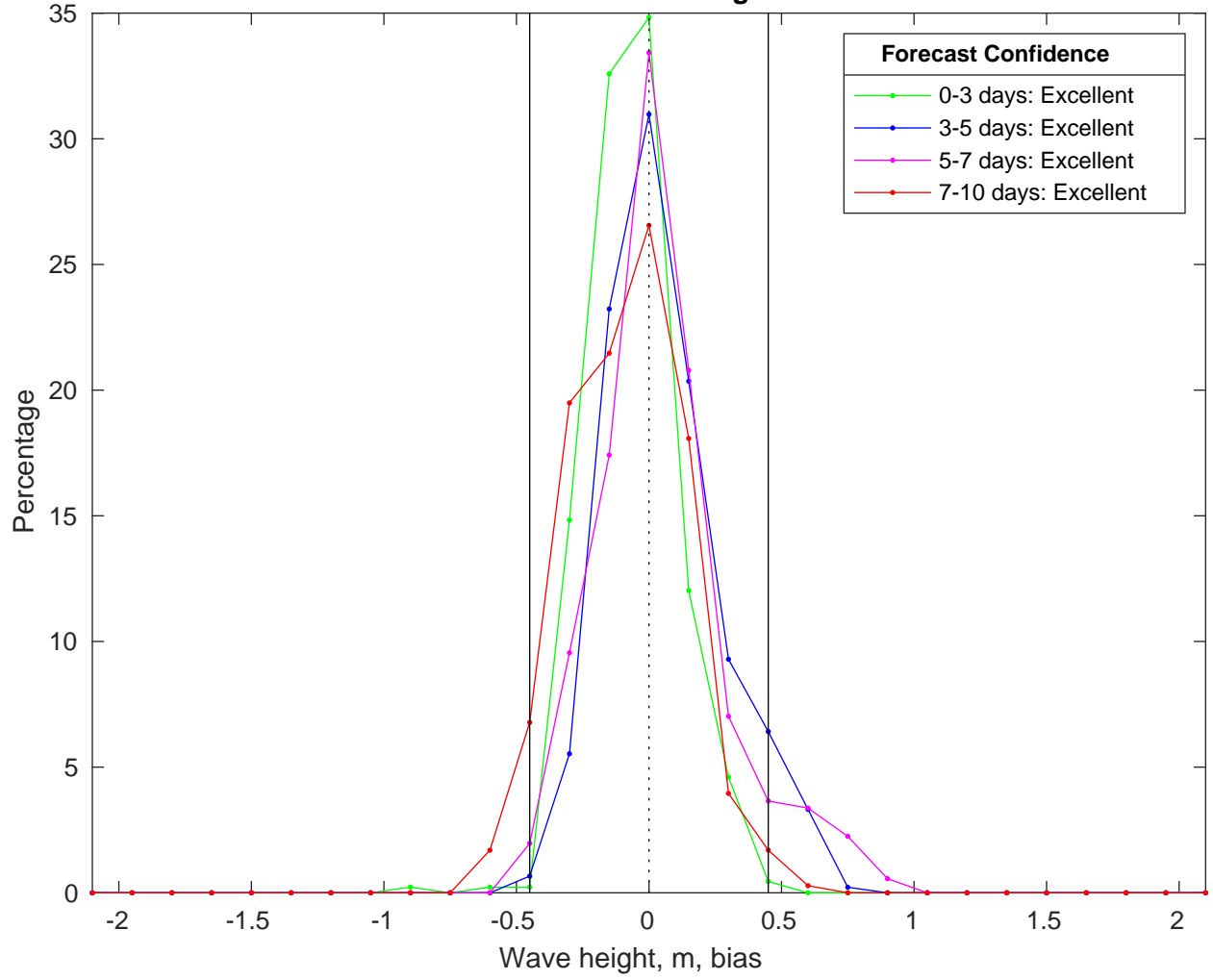
NDBC 52212 vs CMEMS Waves Bias Histogram: 05-Mar-2025
