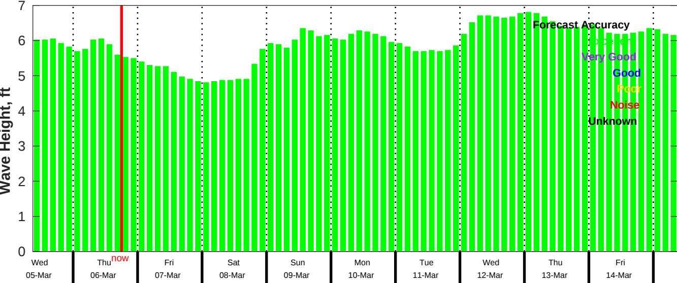
CMEMS Wave Forecast for NDBC 52212 from 04-Mar-2025 09:00:00 to 14-Mar-2025 09:00:00
