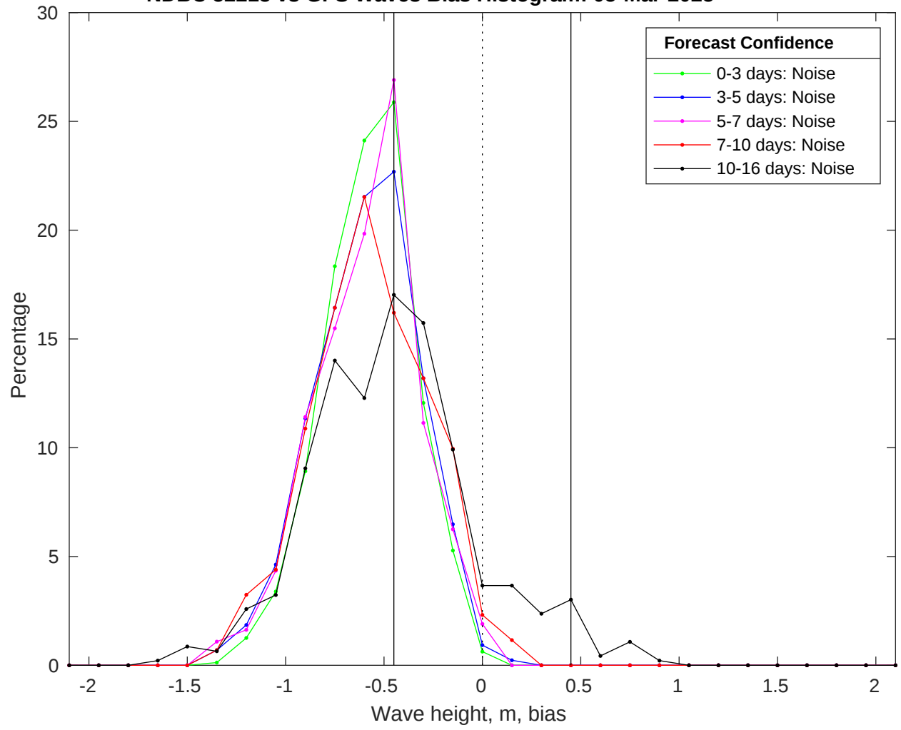
NDBC 52213 vs GFS Waves Bias Histogram: 05-Mar-2025
