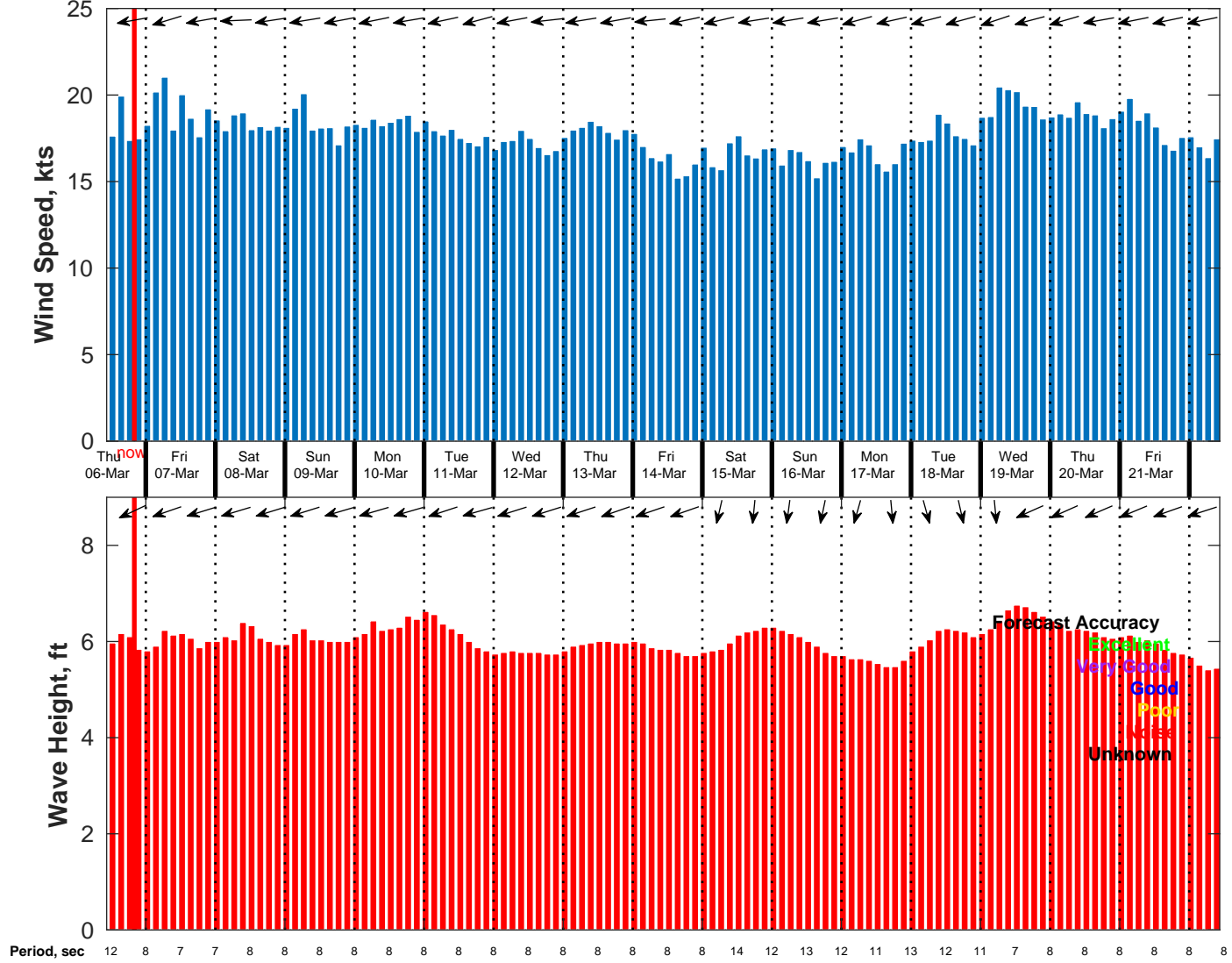
Wind & Wave Forecast for NDBC 52213 from 05-Mar-2025 11:00:00 to 21-Mar-2025 11:00:00
