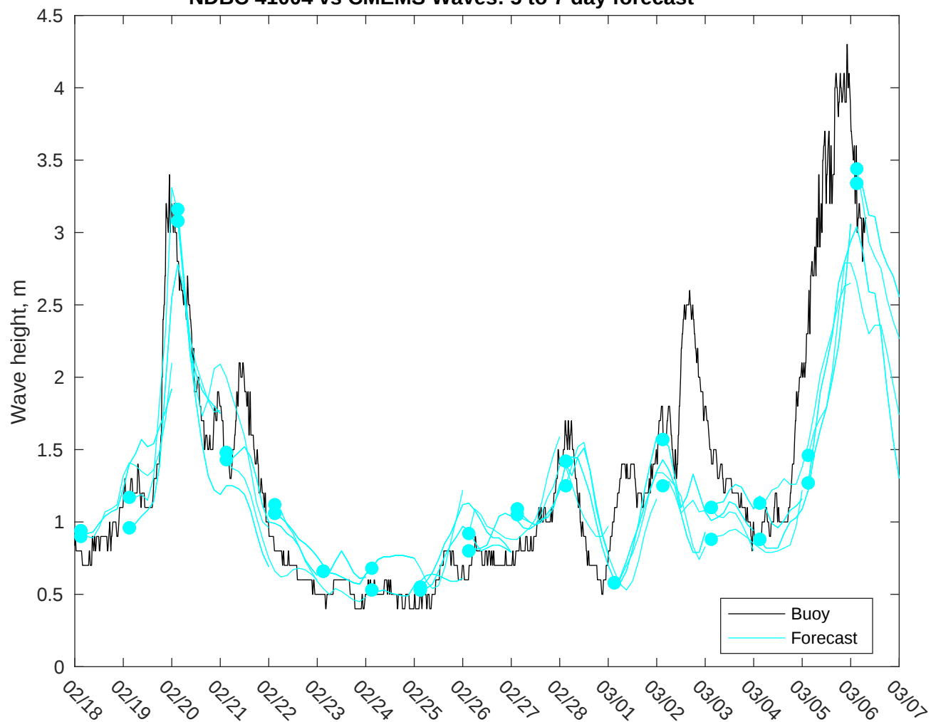
NDBC 41004 vs CMEMS Waves: 5 to 7 day forecast
