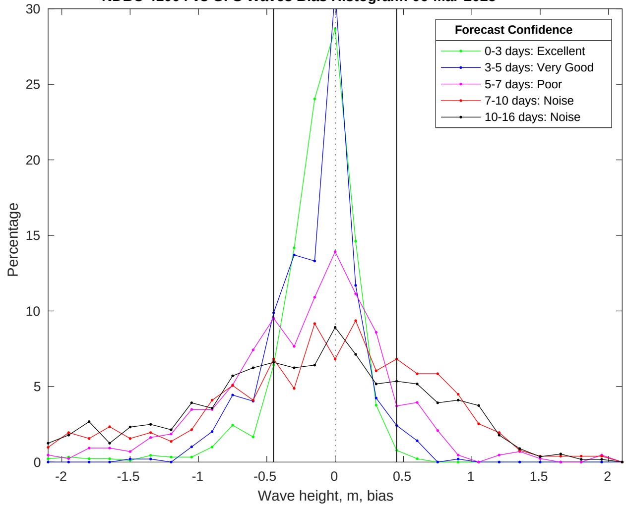
NDBC 41004 vs GFS Waves Bias Histogram: 06-Mar-2025
