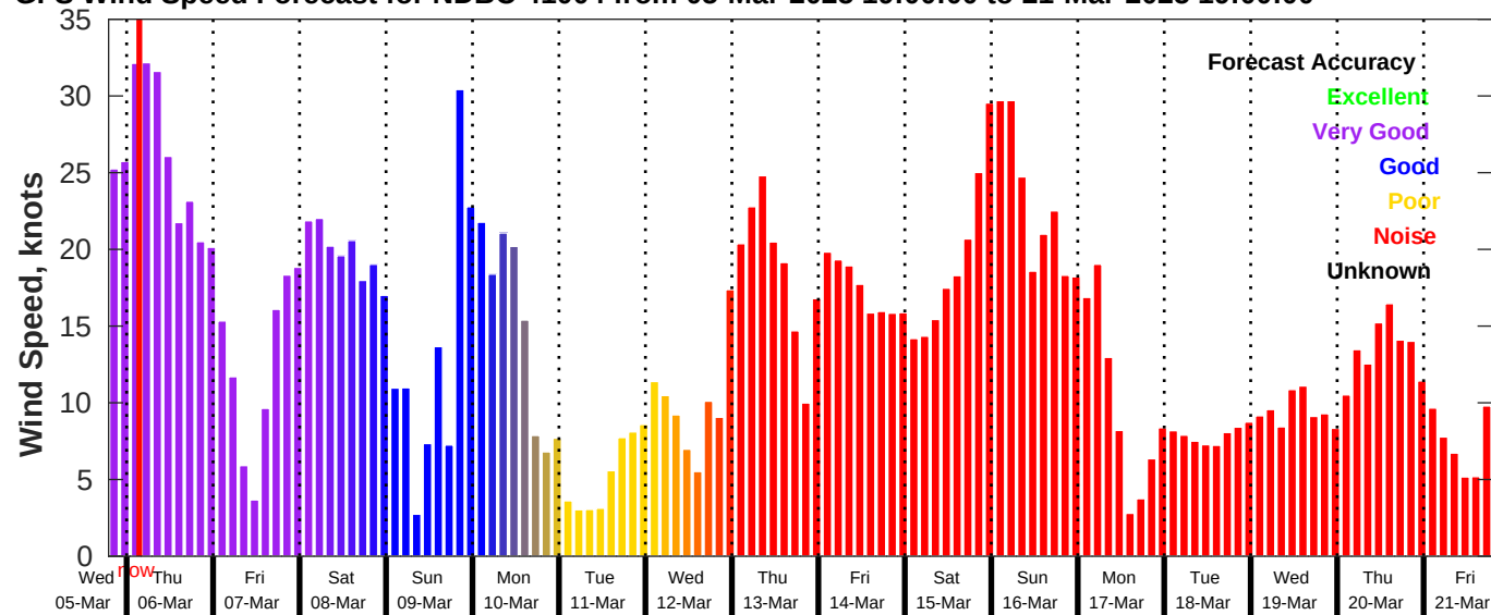
GFS Wind Speed Forecast for NDBC 41004 from 05-Mar-2025 19:00:00 to 21-Mar-2025 19:00:00
