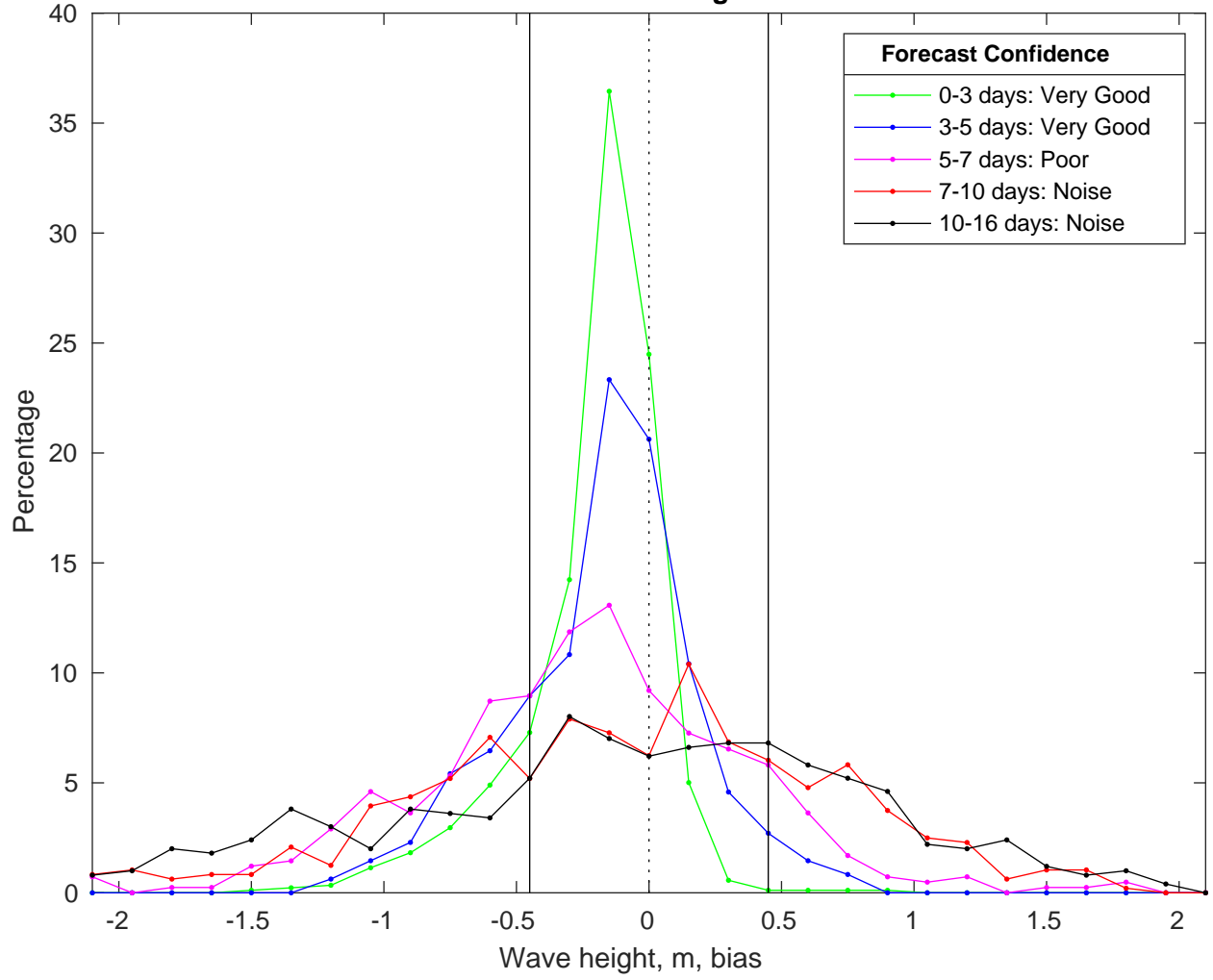
NDBC 41013 vs GFS Waves Bias Histogram: 06-Mar-2025
