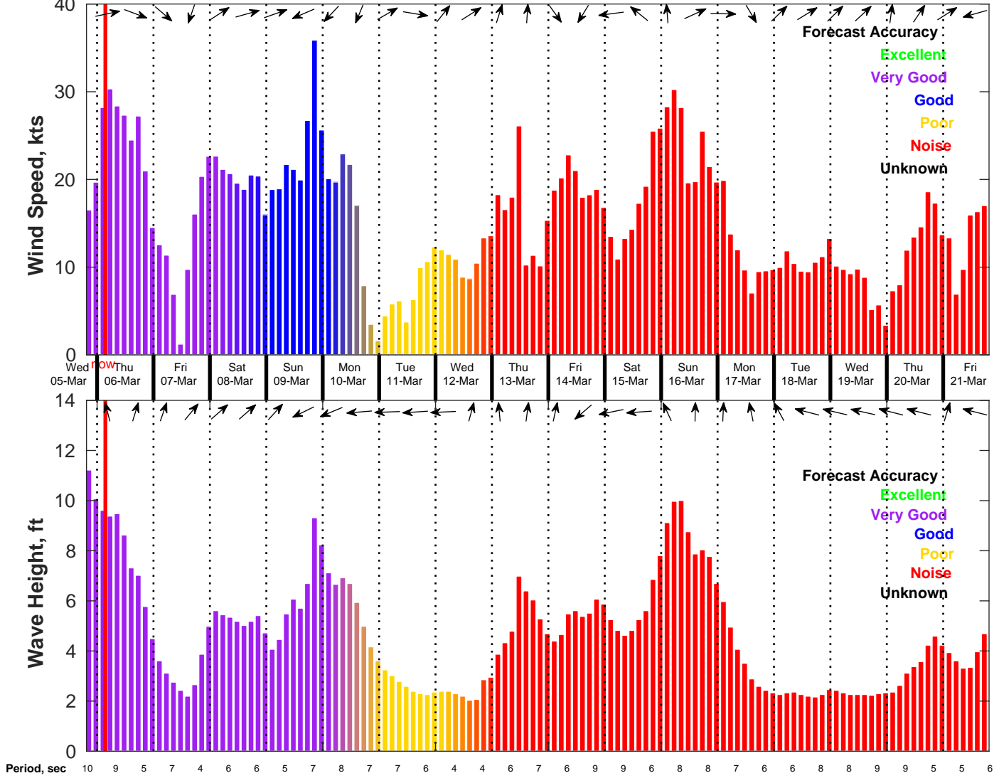
Wind & Wave Forecast for NDBC 41013 from 05-Mar-2025 19:00:00 to 21-Mar-2025 19:00:00
