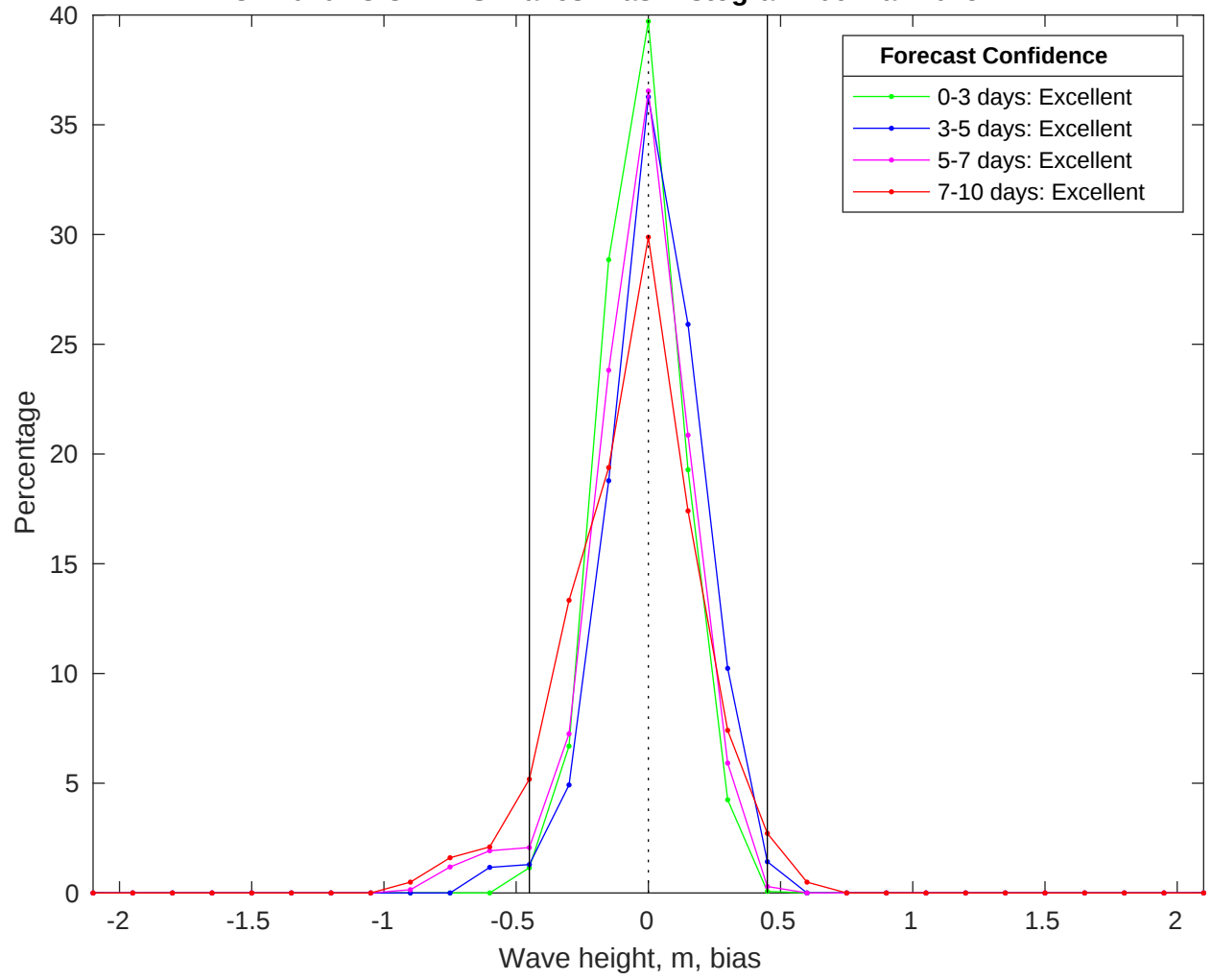
NDBC 41040 vs CMEMS Waves Bias Histogram: 06-Mar-2025
