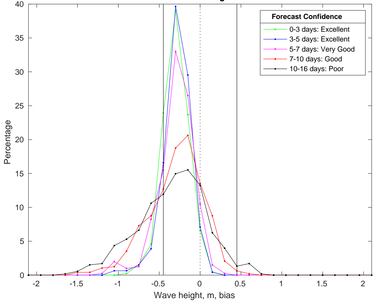
NDBC 41040 vs GFS Waves Bias Histogram: 06-Mar-2025
