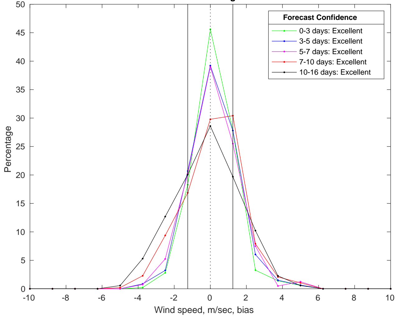
NDBC 41040 vs GFS Winds Bias Histogram: 06-Mar-2025
