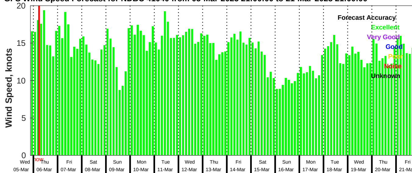
GFS Wind Speed Forecast for NDBC 41040 from 05-Mar-2025 21:00:00 to 21-Mar-2025 21:00:00
