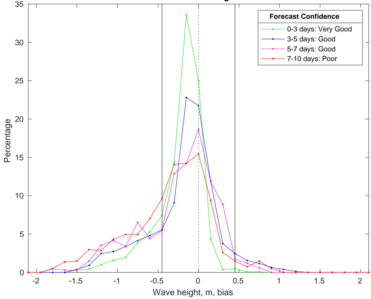
NDBC 42019 vs CMEMS Waves Bias Histogram: 06-Mar-2025
