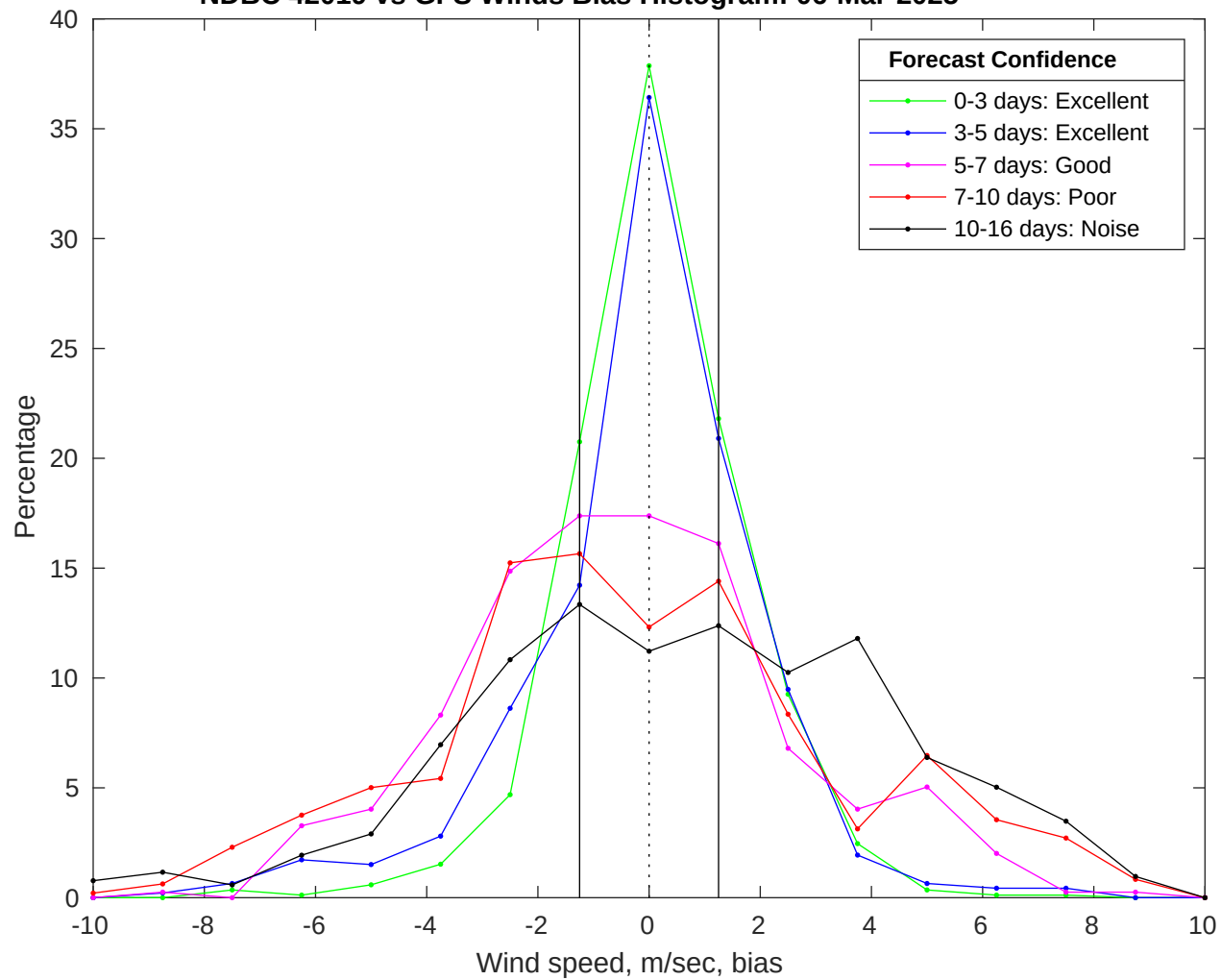
NDBC 42019 vs GFS Winds Bias Histogram: 06-Mar-2025
