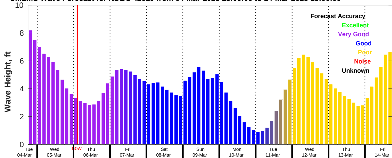
CMEMS Wave Forecast for NDBC 42019 from 04-Mar-2025 18:00:00 to 14-Mar-2025 18:00:00
